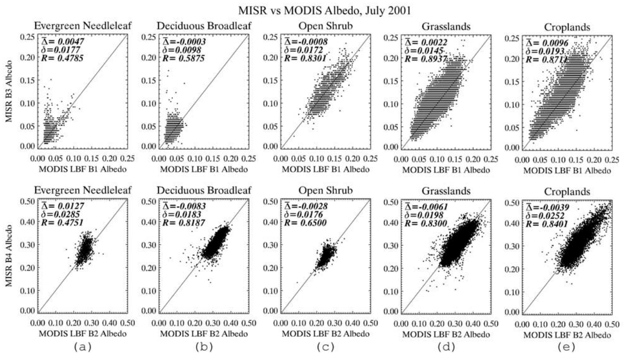
Figure 12. Scatterplots of MISR albedo plotted against MODIS albedo derived by the land cover-based fitting algorithm for two spectral bands ((top) red and (bottom) NIR) for July 2001: (a) evergreen needleleaf forest, (b) deciduous broadleaf forest, (c) open shrublands, (d) grasslands, and (e) croplands.
