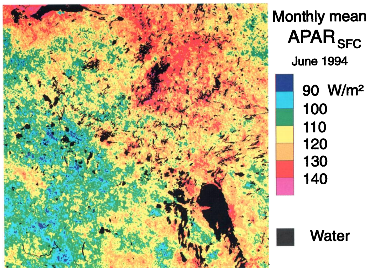
Plate 1. Distribution of monthly mean APAR_{SFC} estimated from AVHRR in the BOREAS region in June 1994. It covers an area of 1000 \times 1000 \text{ km}^2 , centered around 55^{\circ}13'41''\text{N} and 103^{\circ}6'53''\text{W} , with the Lambert conformal conic projection.
