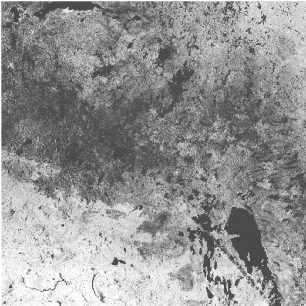
Figure 11. Same as Figure 10 but for minimum AVHRR channel 1 albedo.
