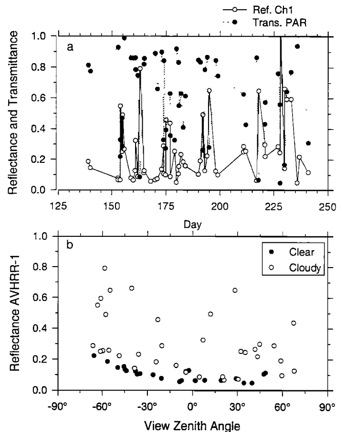
Figure 6. Variation of AVHRR channel 1 reflectance with date and viewing zenith angle over the NOBS in the summer of 1994. Open and solid circles correspond to cloudy and clear measurements.
