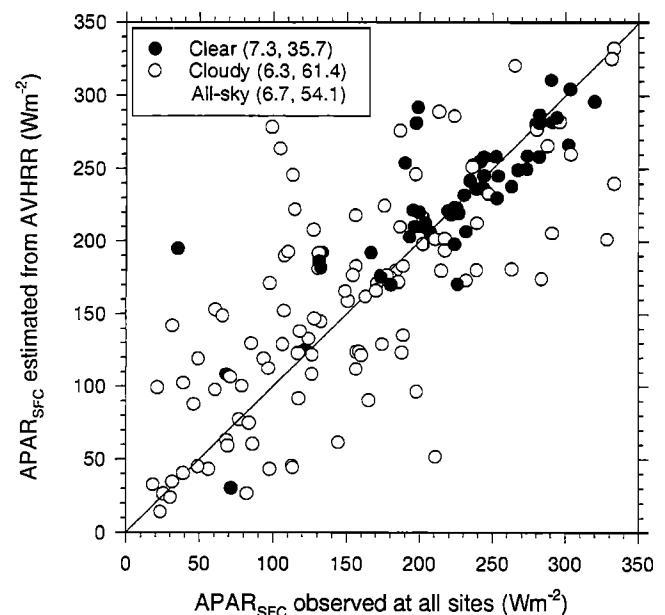
Figure 9. Same as Figure 8 but for all the three towers under study (NOBS, NOJP, and SOBS). The data are differentiated into clear and cloudy.
