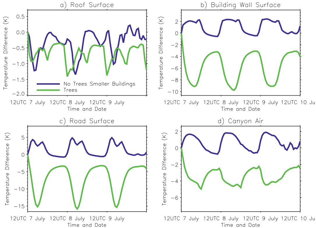
FIG. 6. Time series of no trees/shorter buildings minus no trees (blue), and trees minus no trees (green) simulated subgrid (a) roof-, (b) building-wall-, and (c) road-surface temperatures and (d) canyon air temperature with a horizontal resolution of 0.5 km averaged over all urban land-use categories from the 3-day simulations between 1200 UTC 7 Jul and 1200 UTC 10 Jul 2007.
