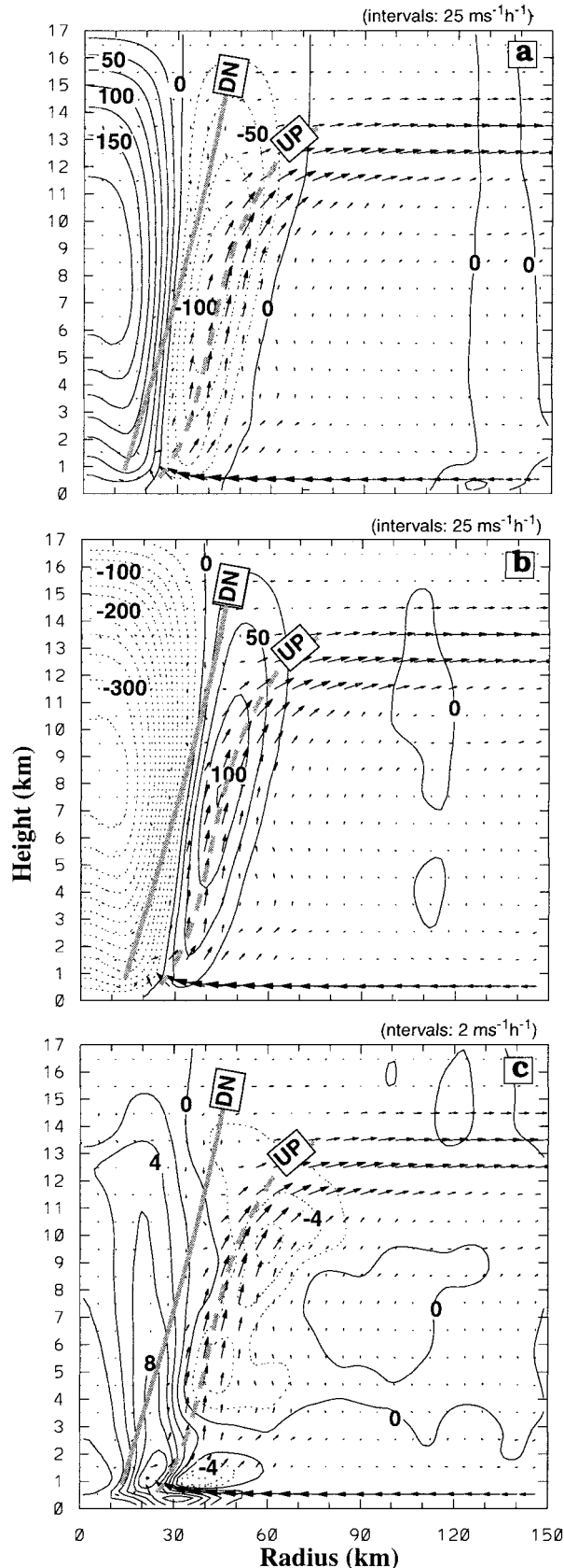
FIG. 10. As in Fig. 1 but for the decomposed components of PGF associated with the term (a) \rho \nabla_k^2 (V_k^2/2) , (b) \rho \nabla_k \cdot (\mathbf{V}_h \times \mathbf{z}_k) , and (c) the residual [see Eq. (7) for definitions].
