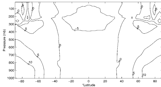
FIG. 18. Change in equilibrium temperature when the surface static stability is increased by 5% and held fixed.
