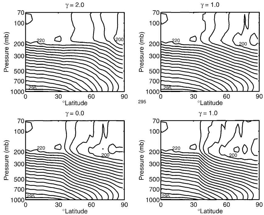
FIG. 15. Contours of temperature plotted vs p and \phi , for various values of \gamma and no overturning circulation. Contour interval 5 K.
