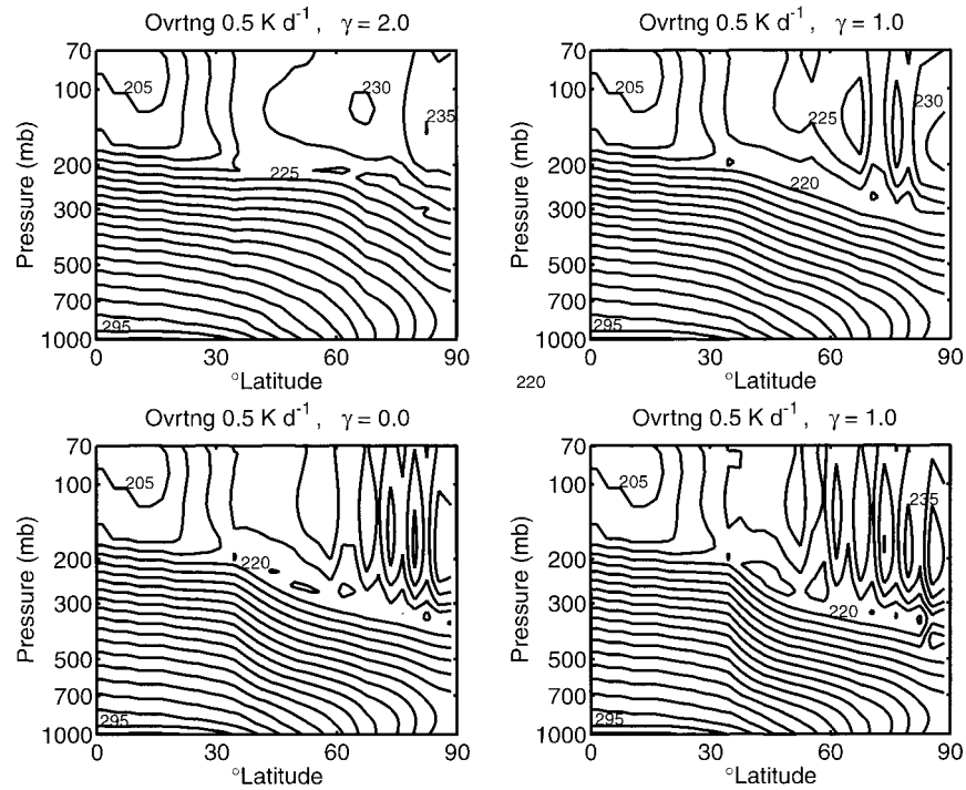
FIG. 14. Contours of temperature plotted vs p and \phi , for various values of \gamma , with standard overturning circulation. Contour interval 5 K.
