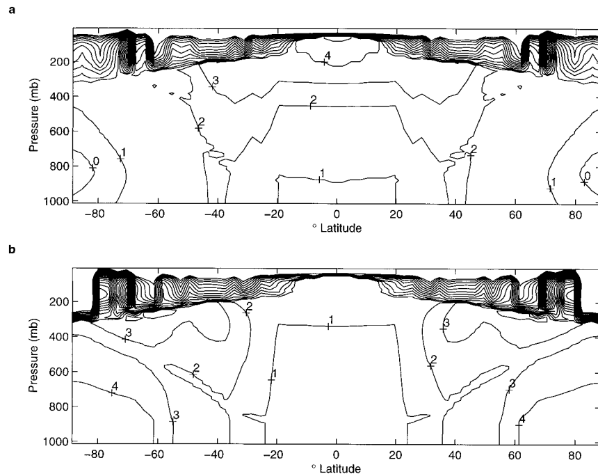
FIG. 21. Change in equilibrium temperature when the concentration of \text{CO}_2 is increased from 300 to 600 ppmv for (a) surface static stability adjusted so that the isentrope leaving the boundary layer at the edge of the Tropics intersects the tropopause at each Pole and (b) constant surface static stability.
