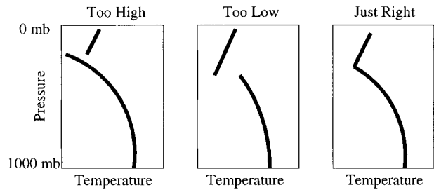
FIG. 5. Schematic depiction of tropopause height determination.
