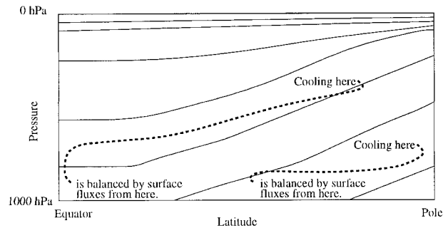
FIG. 7. Schematic of surface turbulent heat flux allocation. Solid lines are isentropes. Radiative heating on a given isentrope in the free troposphere is balanced by heat and moisture fluxes from the surface in the region where that isentrope intersects the surface. If the isentrope never intersects the surface, radiative cooling is balanced by convective heat fluxes that are initially assumed to take place in the Tropics only.
