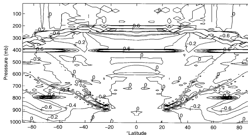
FIG. 19. Change in equilibrium radiative heating rate when the surface static stability is increased by 5% and held fixed.
