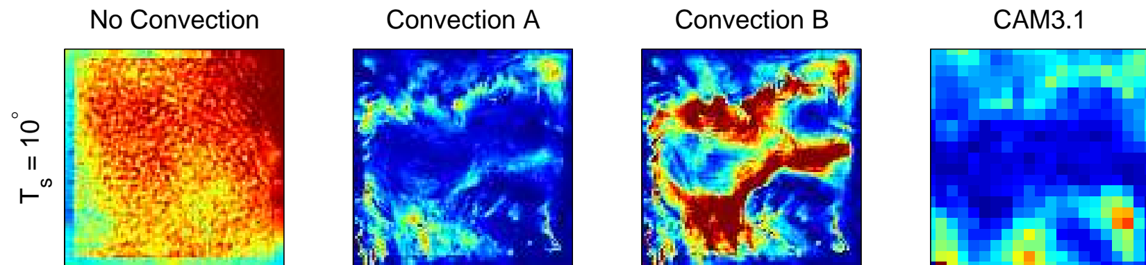
908 hPa Cloud Water (0 — 150 ppm)
