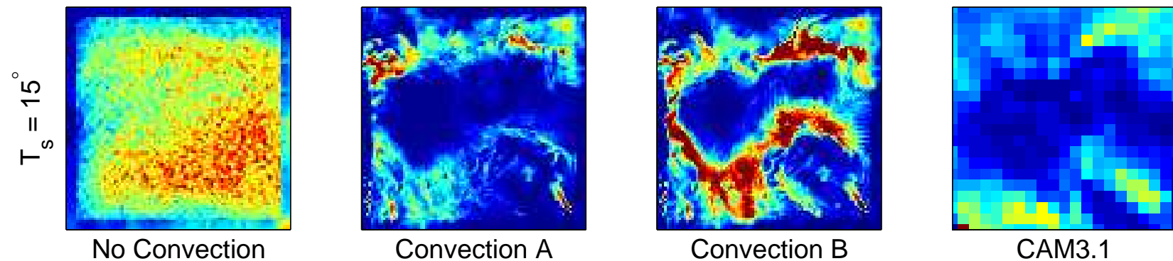
908 hPa Cloud Water (0 — 150 ppm)
