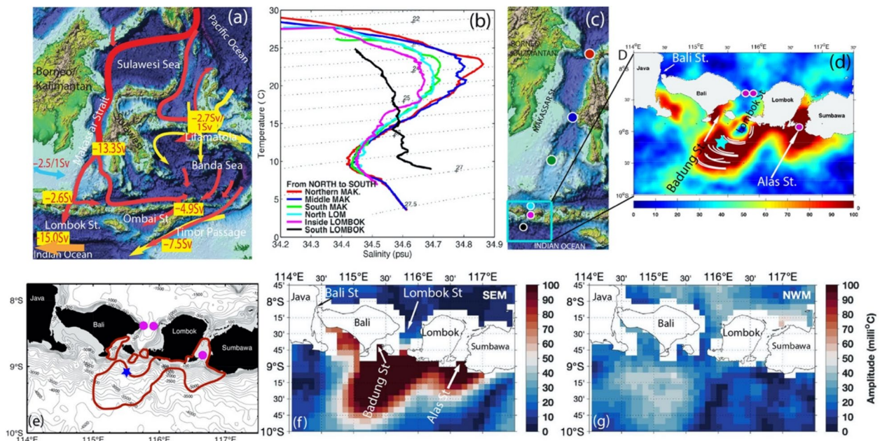
Fig. 1 a Map of the main Indonesian throughflow (ITF) pathways in the eastern part of Indonesia from the Pacific into the Indian Ocean. b Temperature–salinity (TS) diagram of the evolution of water masses from north of Makassar Strait through Lombok Strait into the Indian Ocean taken during the TRIUMPH (ThRoughflow Indonesian seas, Upwelling, and Mixing PHYSics) cruise in December 2019, revealing strong mixing in Makassar and Lombok Straits for potential densities \sigma_{\theta}=23\text{--}27\text{ kg m}^{-3} (modified from Susanto and Ray 2022). c Map of the Makassar and Lombok Straits showing the location of the stations used in (b). d Estimates of fortnightly ( MS_f ) SST amplitude in ^{\circ}\text{C} (Susanto and Ray 2022; Ray and Susanto 2016). White lines in the SST anomaly south of Lombok Strait coincide with soliton signatures observed by SAR satellites (Susanto et al. 2005; Matthews et al. 2011). The high SST amplitudes in d are consistent with tidal mixing which we hypothesize is responsible for the abrupt changes in the T–S diagram from inside to the south of Lombok Strait indicate strong mixing as waters pass over the sills at the southern end of Lombok Strait seen in (b). e Map of the Lombok Strait showing the locations of the TRIUMPH ITF moorings (purple circles) and mixing measurements (blue star). The north entrance of the Lombok Strait is 1200-m deep and 35-km wide. The sill is 300-m deep and 22-km wide. Badung Sill is 105-m deep and 19-km wide. Alas Strait is 150-m deep and 21-km wide and Bali Strait is 70-m deep and 8-km wide. Gray lines are bathymetry contours. The red lines are the 80 ^{\circ}\text{C} fortnightly signal ( MS_f ) sea surface temperature (SST) amplitude contour from (c). f, g Estimates of fortnightly ( MS_f ) SST amplitude in ^{\circ}\text{C} during the southeast and northwest monsoon, respectively (Susanto and Ray 2022)
