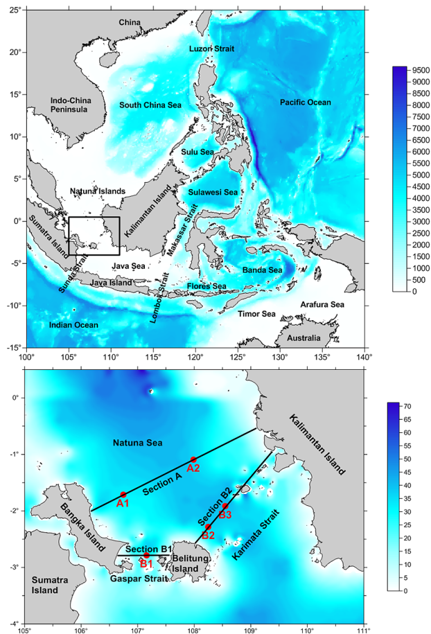
Figure 1. The map of the Indonesian seas (upper), and observational stations (lower). Isobaths are in meters.
