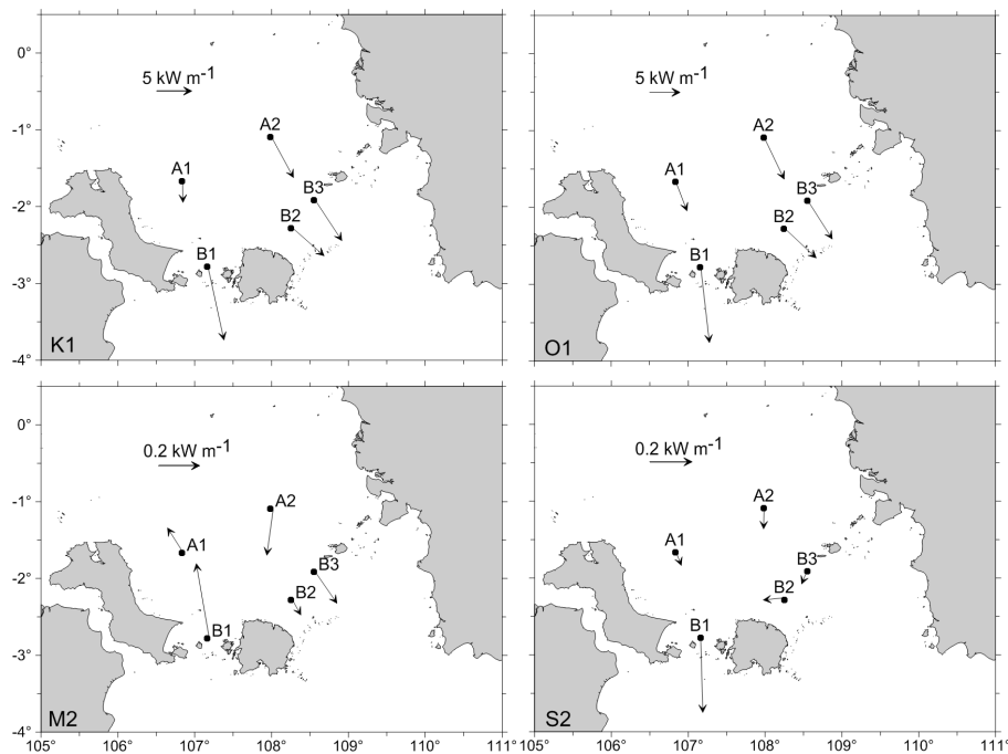
Figure 3. Horizontal tidal energy flux density.
