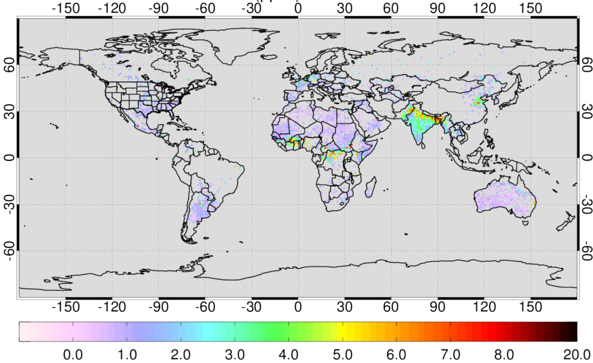
AIRS NH3 VMR (ppbv) at 840hPa for 201103
