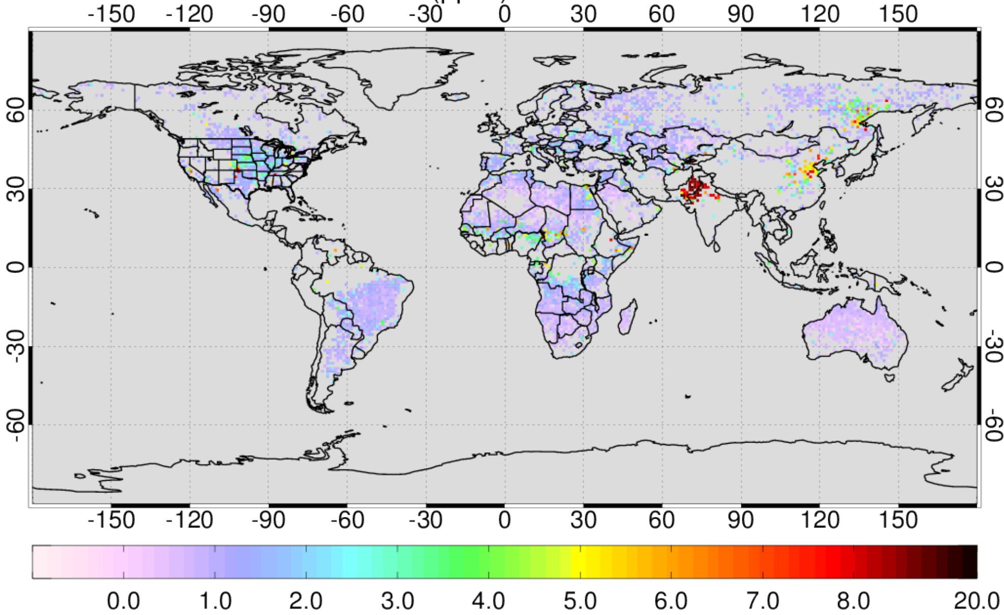
AIRS NH3 VMR (ppbv) at 840hPa for 201107
