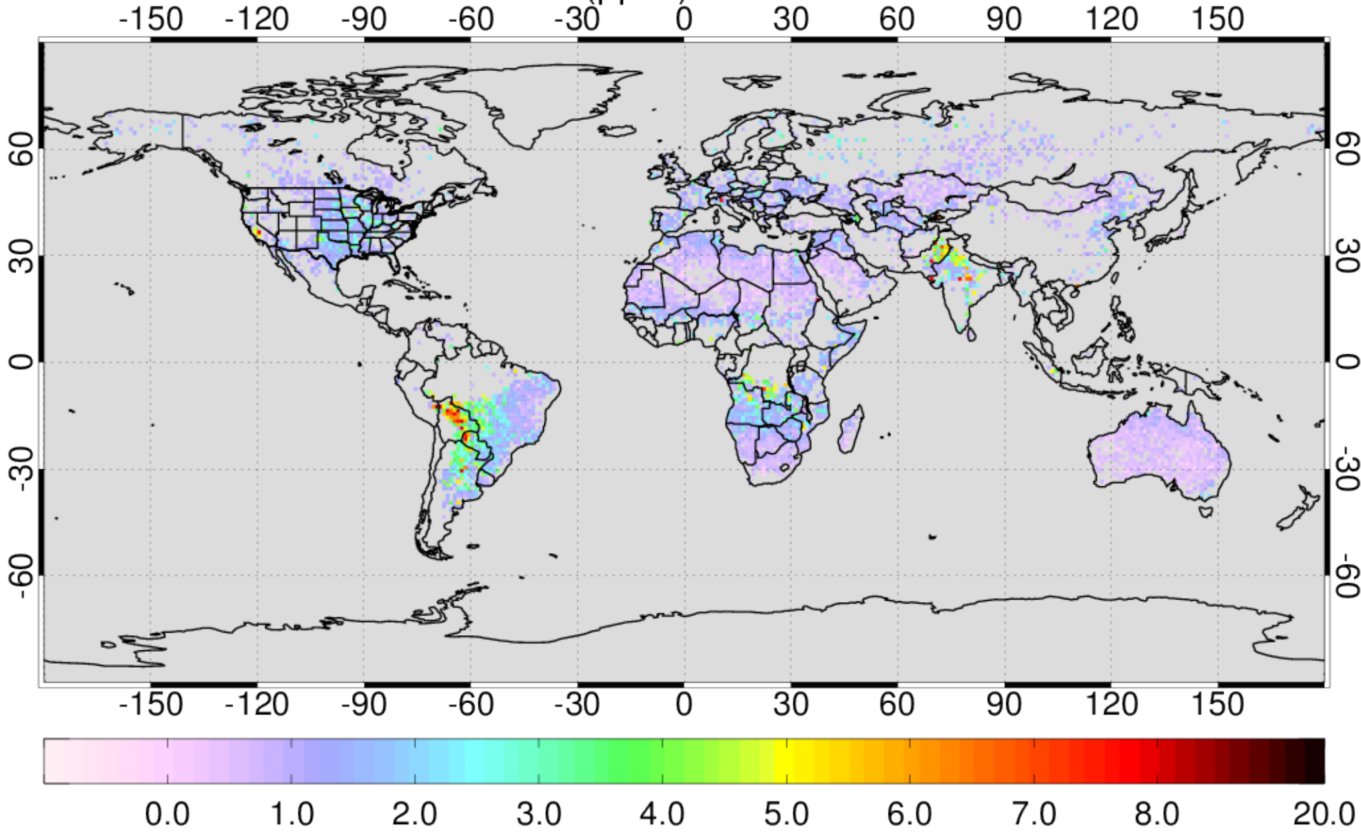
AIRS NH3 VMR (ppbv) at 840hPa for 201109
