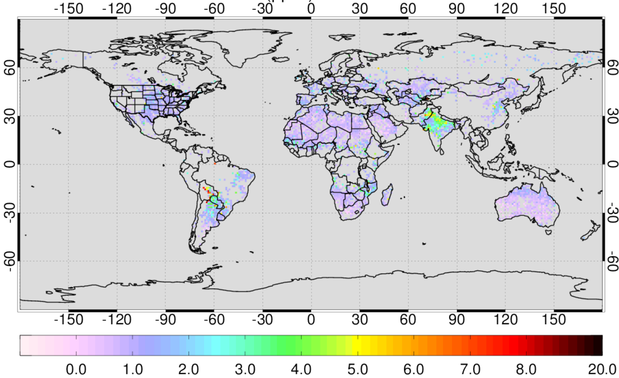
AIRS NH3 VMR (ppbv) at 840hPa for 201110
