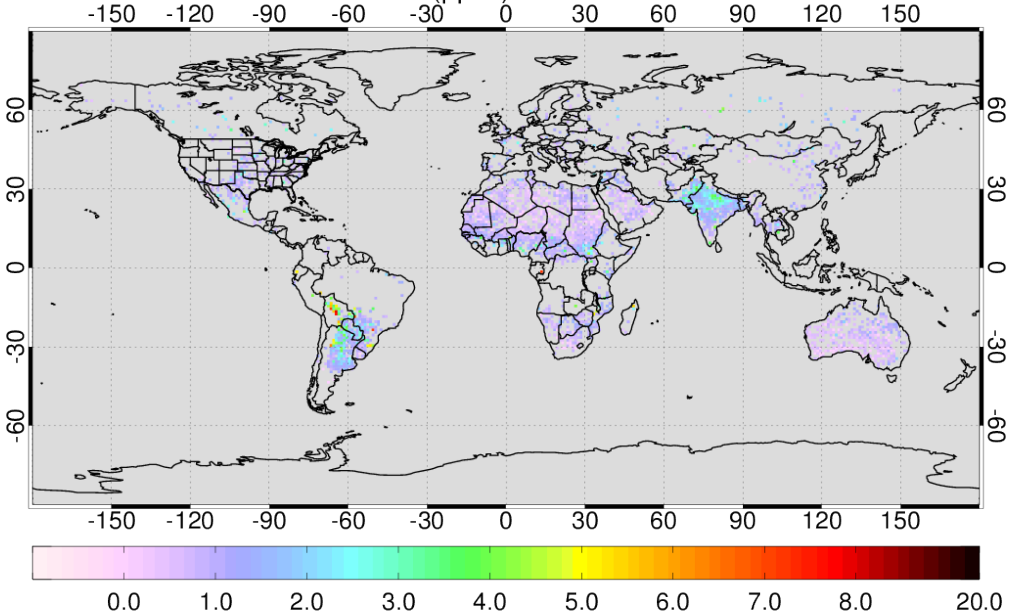
AIRS NH3 VMR (ppbv) at 840hPa for 201111
