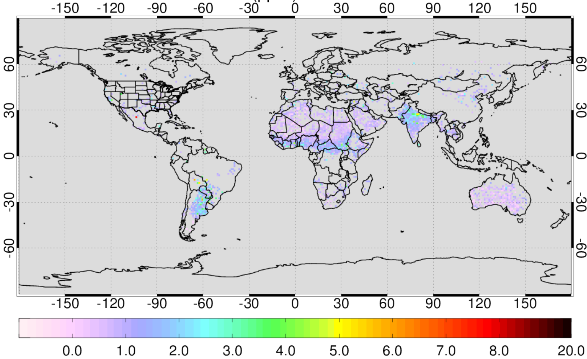
AIRS NH3 VMR (ppbv) at 840hPa for 201112
