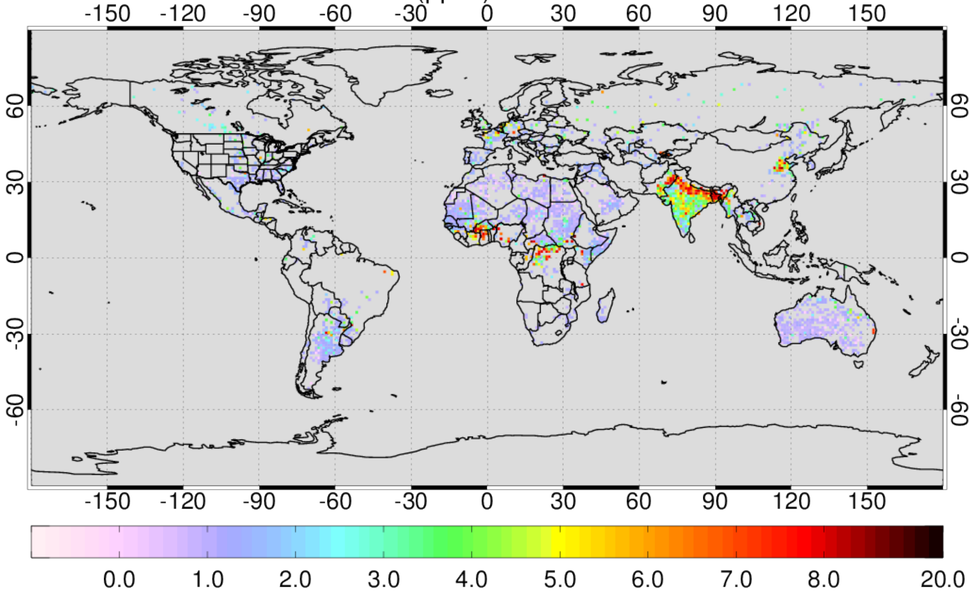
AIRS NH3 VMR (ppbv) at 918hPa for 201103
