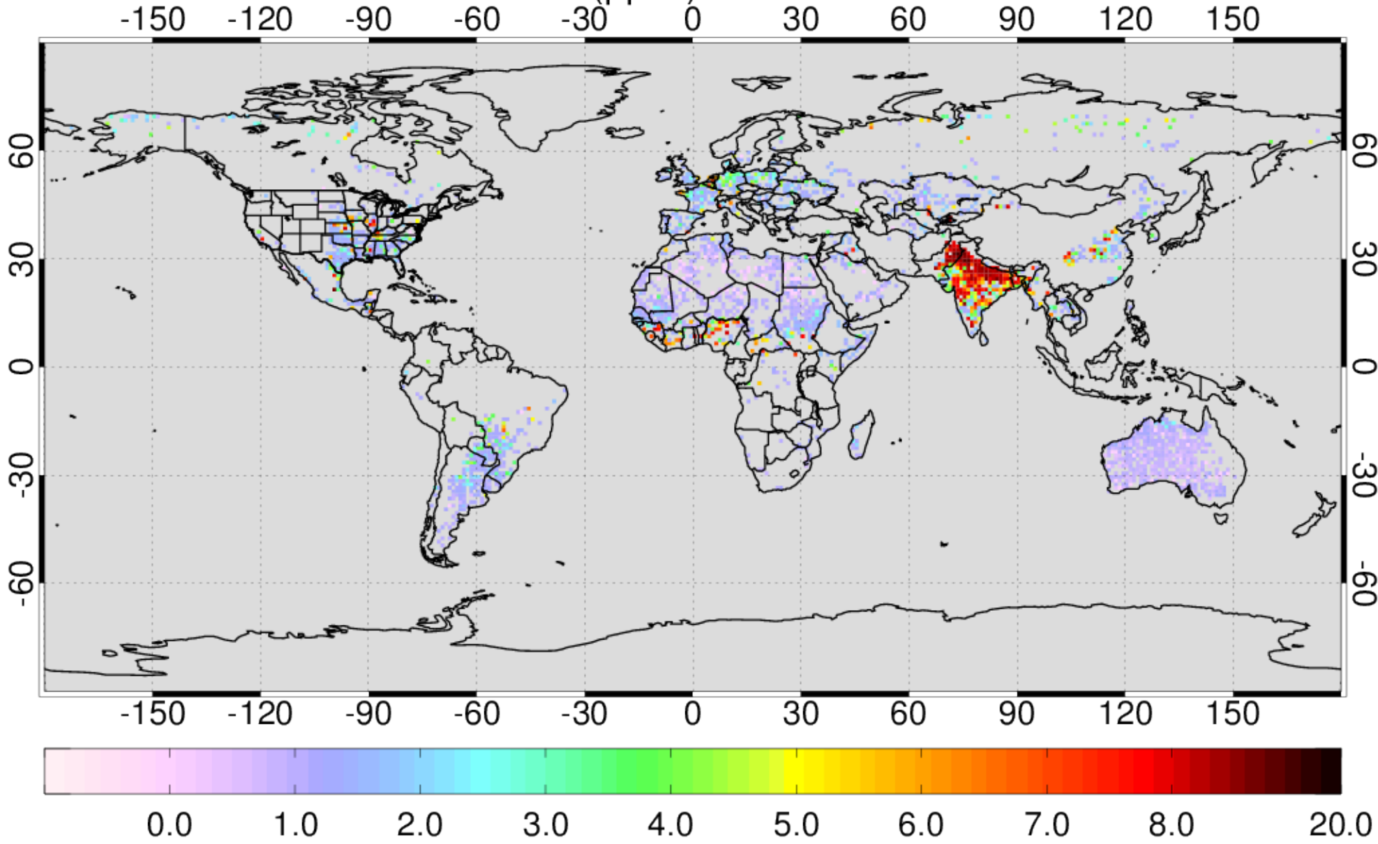
AIRS NH3 VMR (ppbv) at 918hPa for 201104
