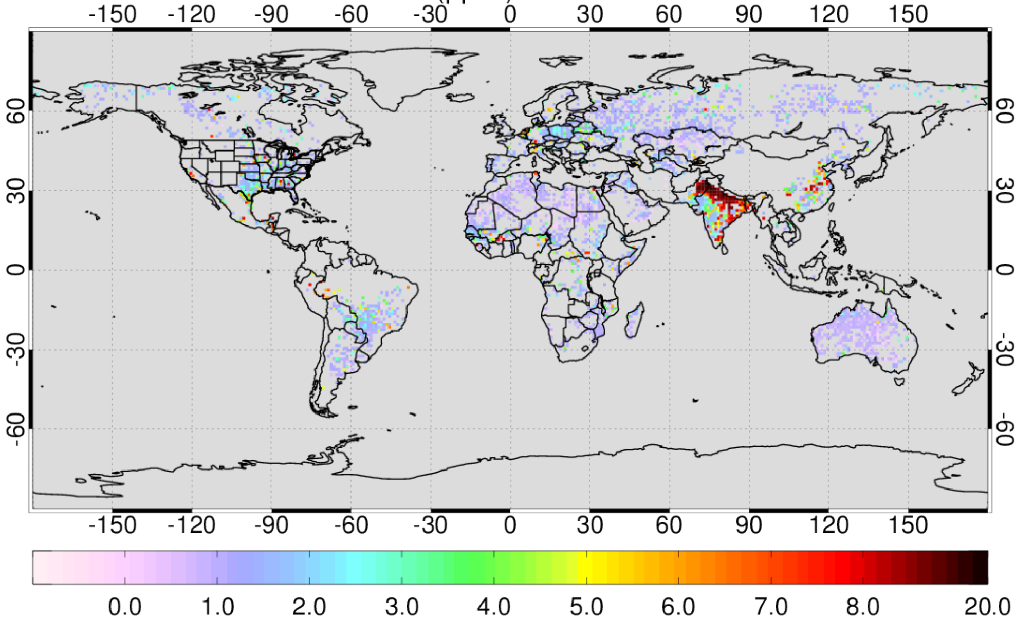
AIRS NH3 VMR (ppbv) at 918hPa for 201105
