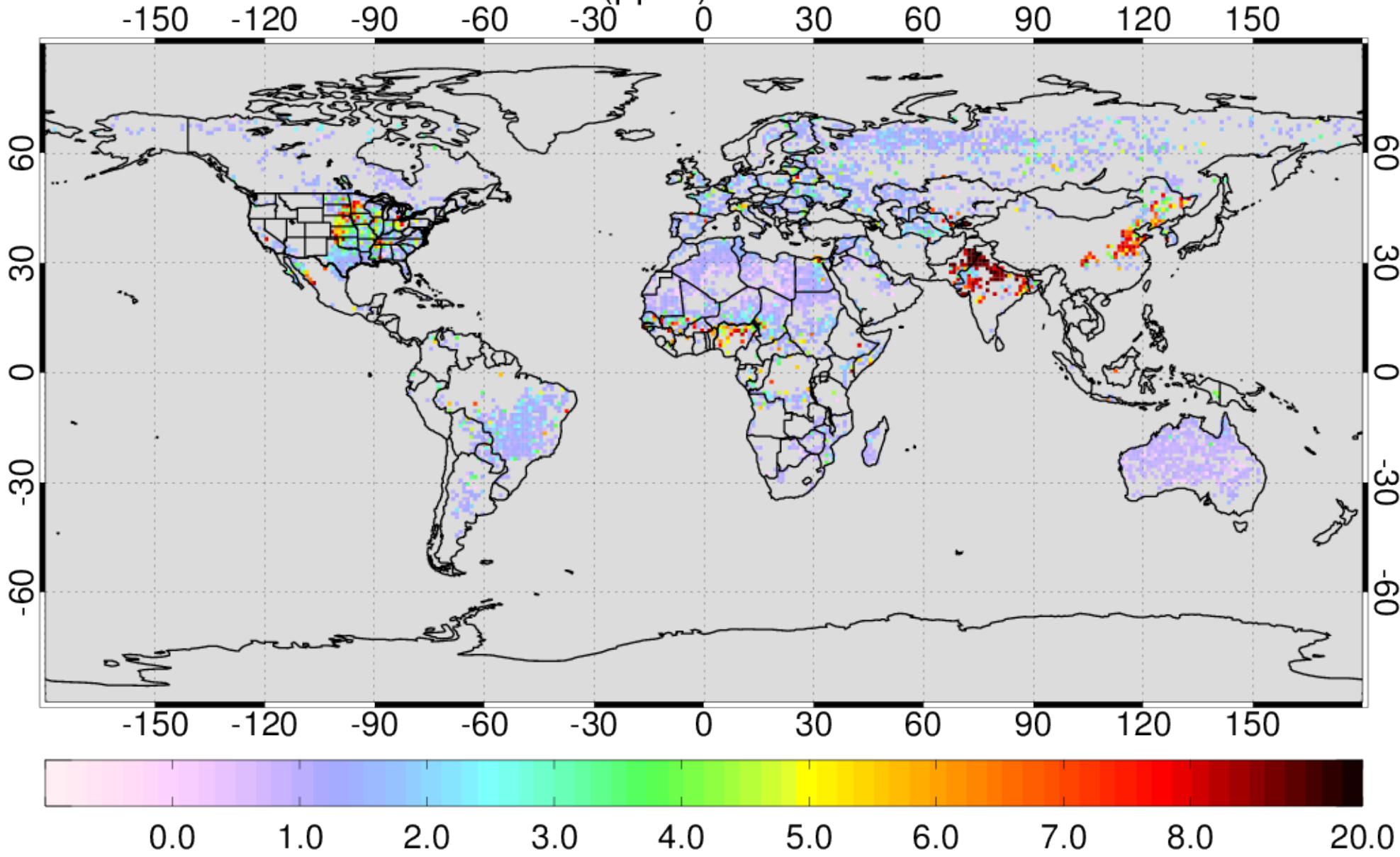
AIRS NH3 VMR (ppbv) at 918hPa for 201106
