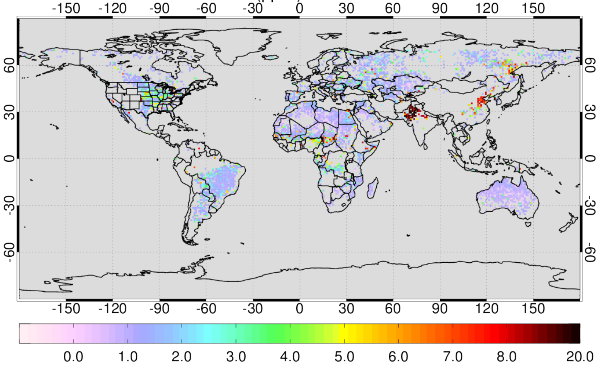
AIRS NH3 VMR (ppbv) at 918hPa for 201107
