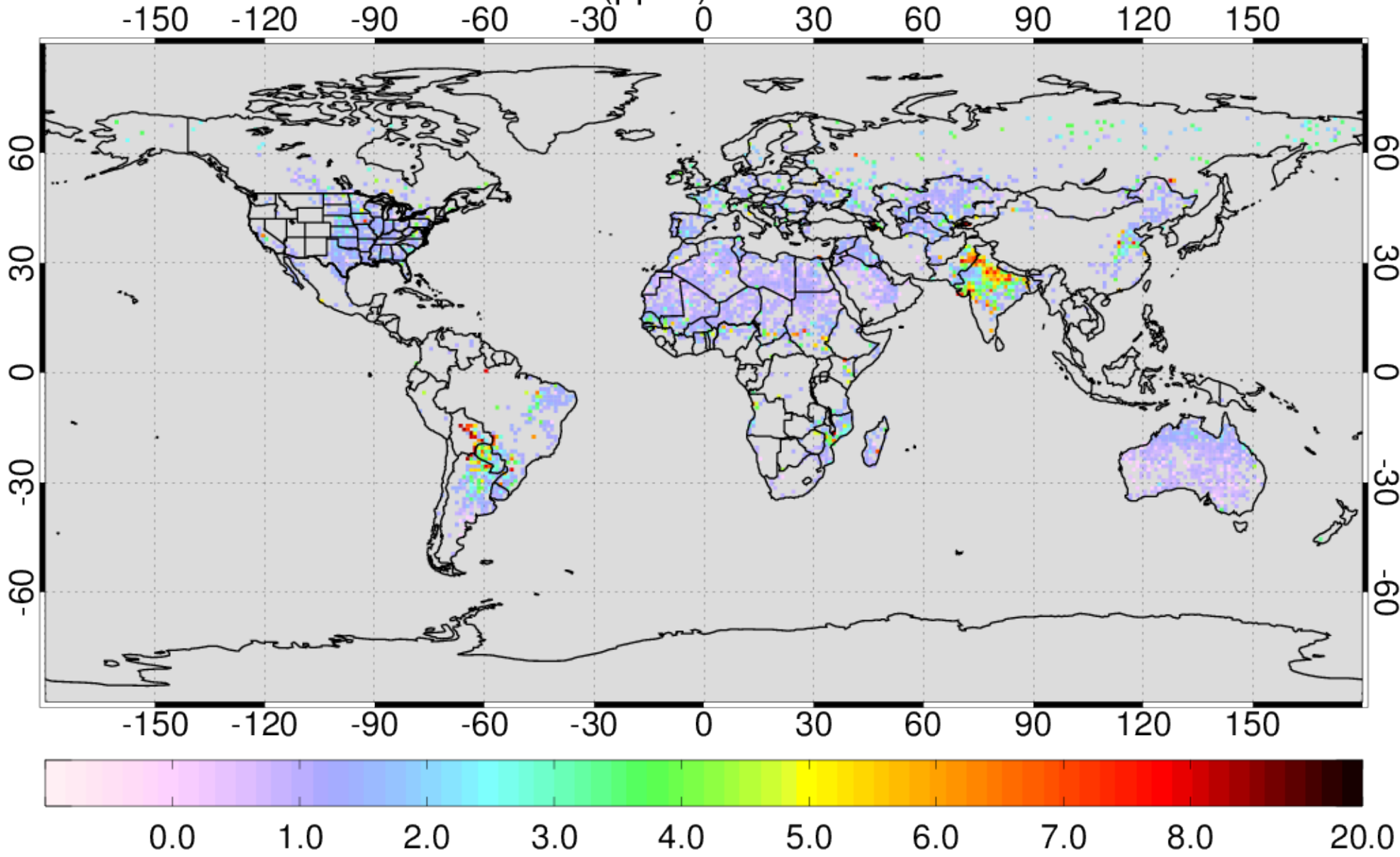
AIRS NH3 VMR (ppbv) at 918hPa for 201110
