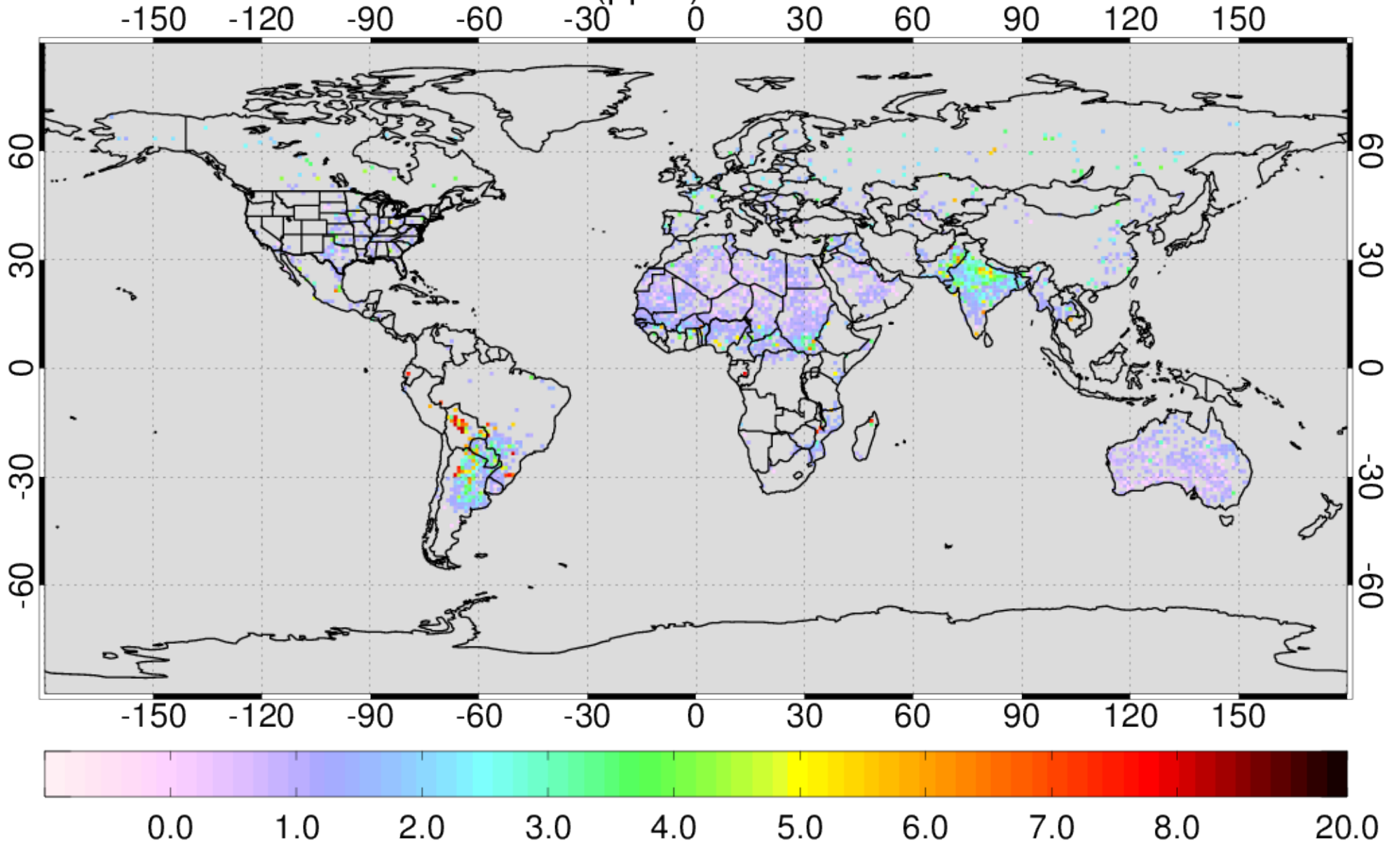
AIRS NH3 VMR (ppbv) at 918hPa for 201111
