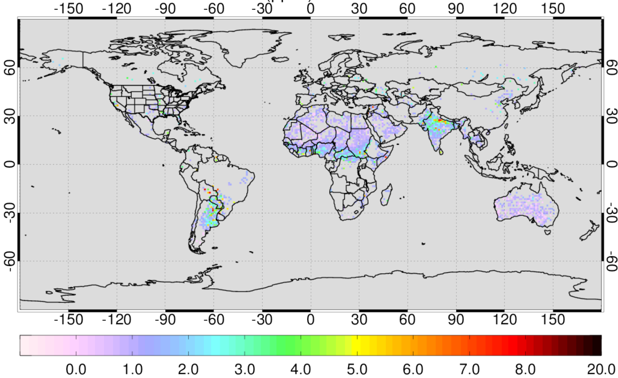
AIRS NH3 VMR (ppbv) at 918hPa for 201112
