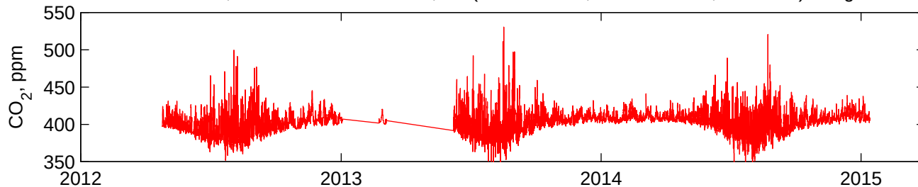
CARBON DIOXIDE, 20 min means. Bremen, IN. (41.457927°N, 86.193528°W, 251m asl). Height 50m agl.
