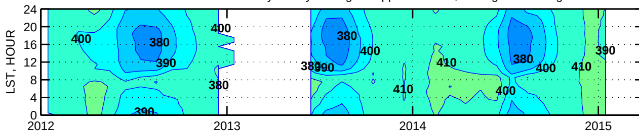
CARBON DIOXIDE Monthly/Hourly averages in ppm. Bremen, IN. Height=100m agl
