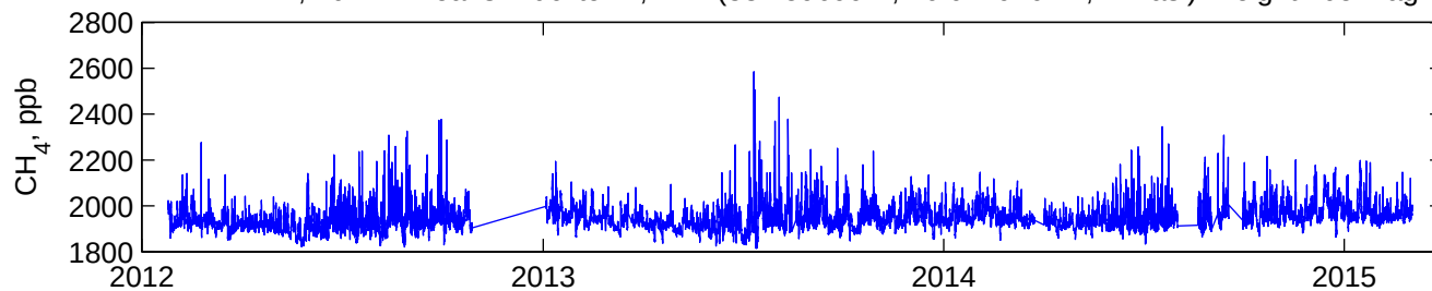
METHANE, 20 min means. Bucktown, MD. (38.45969°N, 76.042970°W, 2m asl). Height 105m agl.
