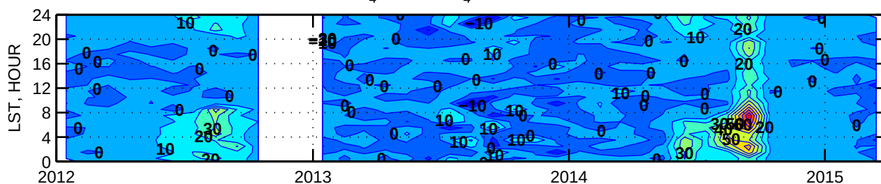
Difference \text{CH}_4(105\text{m}) - \text{CH}_4(50\text{m}) in ppb. Bucktown, MD
