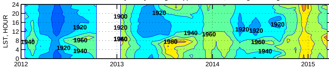
METHANE Monthly/Hourly averages in ppb. Bucktown, MD. Height=50m agl
