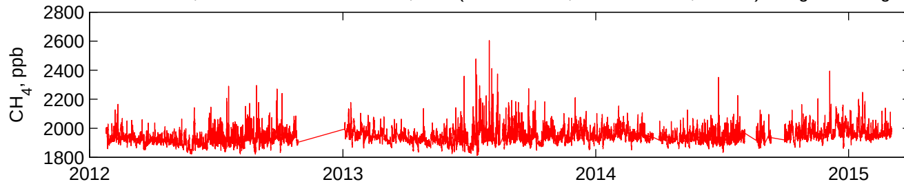
METHANE, 20 min means. Bucktown, MD. (38.45969°N, 76.042970°W, 2m asl). Height 50m agl.
