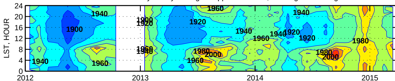
METHANE Monthly/Hourly averages in ppb. Bucktown, MD. Height=105m agl
