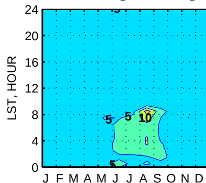
Bucktown, MD. STD CO 2 (105m)-CO 2 (50m), ppm.
