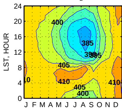
Bucktown, MD. CO 2 (105m), ppm.
