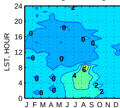
Bucktown, MD. CO 2 (105m)-CO 2 (50m), ppm.
