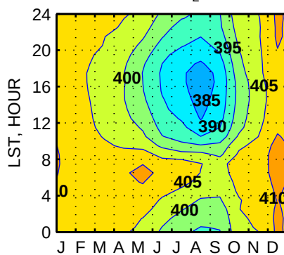
Bucktown, MD. CO 2 (50m), ppm.
