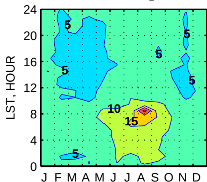
Bucktown, MD. STD CO 2 (105m), ppm.
