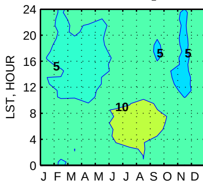
Bucktown, MD. STD CO 2 (50m), ppm.
