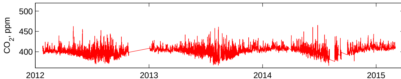
CARBON DIOXIDE, 20 min means. Bucktown, MD. (38.459699°N, 76.042970°W, 2m asl). Height 50m agl.
