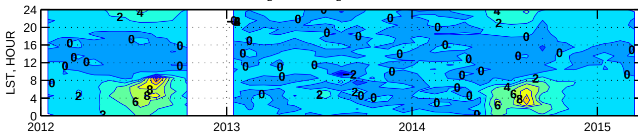
Difference CO 2 (105m)-CO 2 (50m) in ppb. Bucktown, MD
