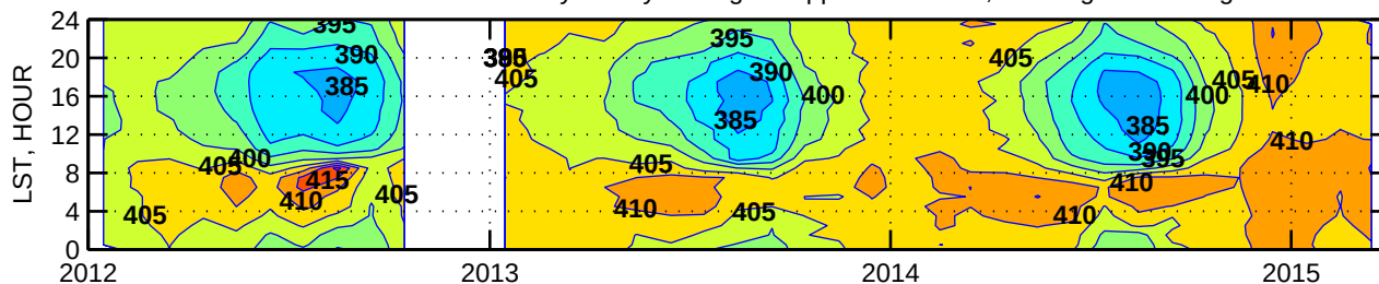
CARBON DIOXIDE Monthly/Hourly averages in ppm. Bucktown, MD. Hight=105m agl
