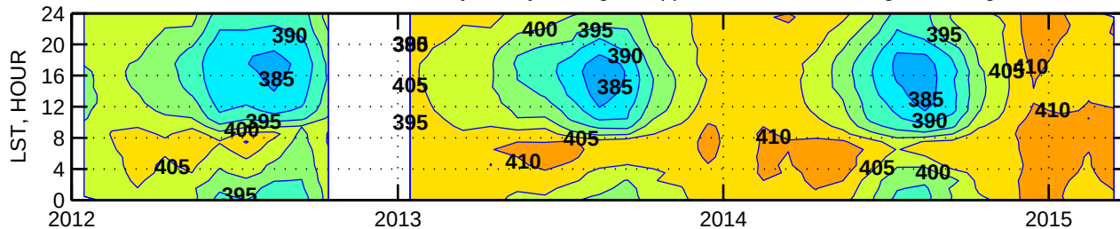
CARBON DIOXIDE Monthly/Hourly averages in ppm. Bucktown, MD. Hight=50m agl
