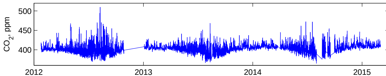
CARBON DIOXIDE, 20 min means. Bucktown, MD. (38.459699°N, 76.042970°W, 2m asl). Height 105m agl.
