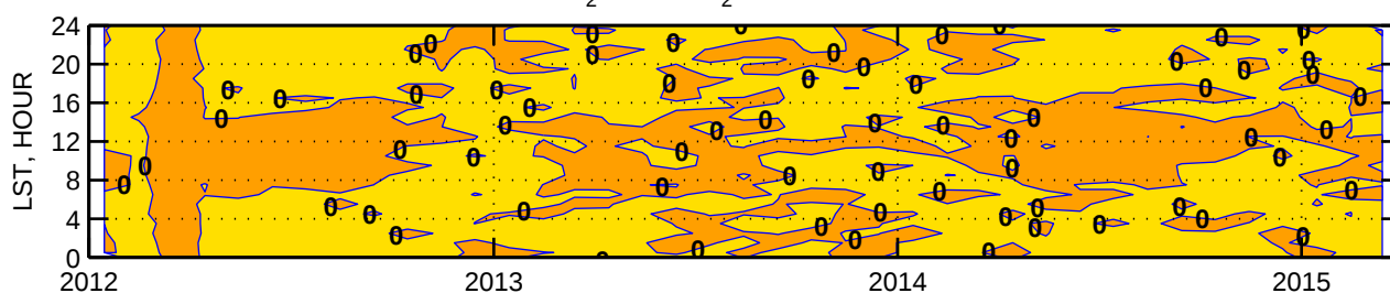
Difference CO 2 (53m)-CO 2 (42m) in ppm. Stockholm, NJ
