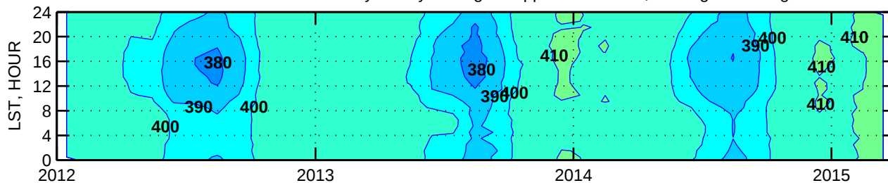
CARBON DIOXIDE Monthly/Hourly averages in ppm. Stockholm, NJ. Height=42m agl
