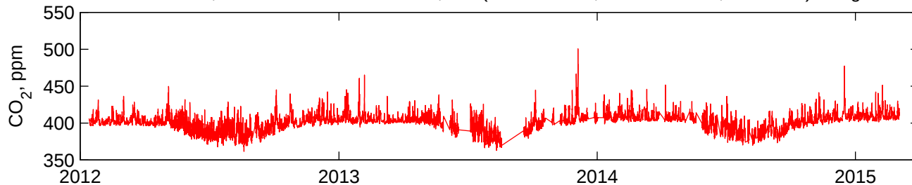
CARBON DIOXIDE, 20 min means. Stockholm, NJ. (41.143556°N, 74.538718°W, 402m asl). Height 42m agl.
