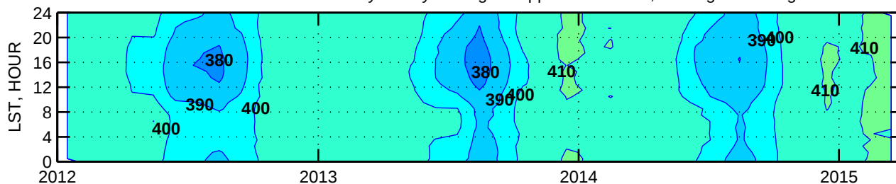
CARBON DIOXIDE Monthly/Hourly averages in ppm. Stockholm, NJ. Height=53m agl
