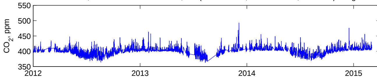
CARBON DIOXIDE, 20 min means. Stockholm, NJ. (41.143556°N, 74.538718°W, 402m asl). Height 53m agl.
