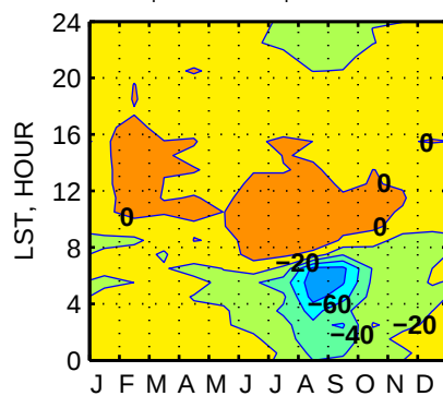
CH 4 (95m)-CH 4 (50m), ppb.
