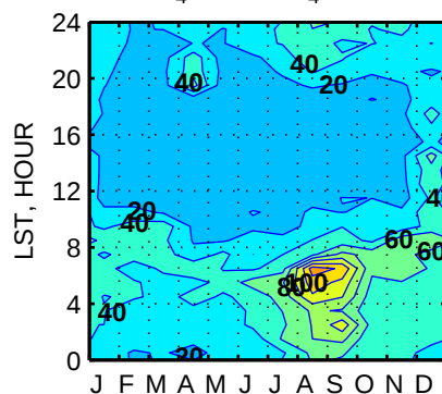
STD CH 4 (95m)-CH 4 (50m), ppb.
