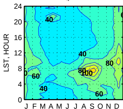
STD CH 4 (95m), ppb.
