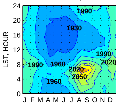
Lewisburg, PA. CH 4 (50m), ppb
