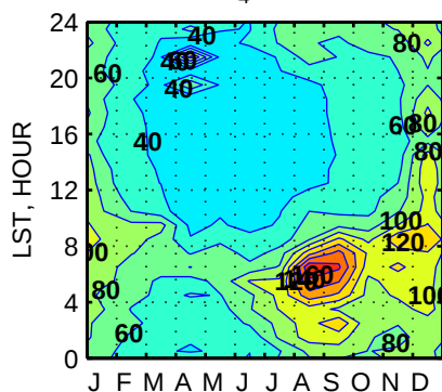
STD CH 4 (50m), ppb.
