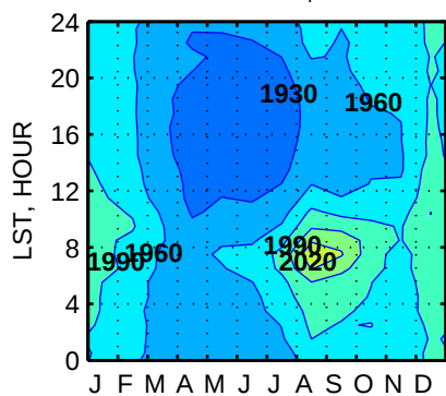
Lewisburg, PA. CH 4 (95m), ppb.
