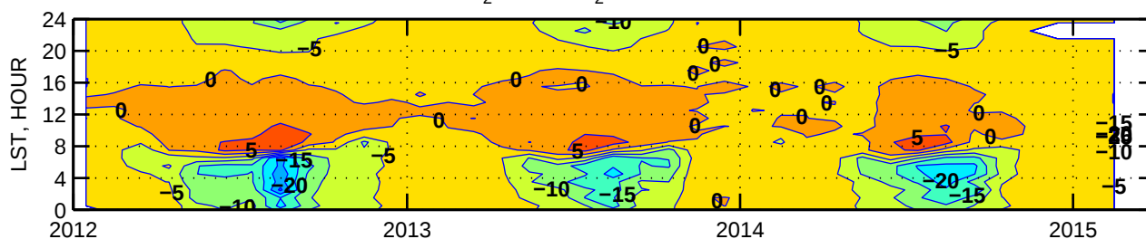
Difference CO 2 (95m)-CO 2 (50m) in ppm. Lewisburg, PA
