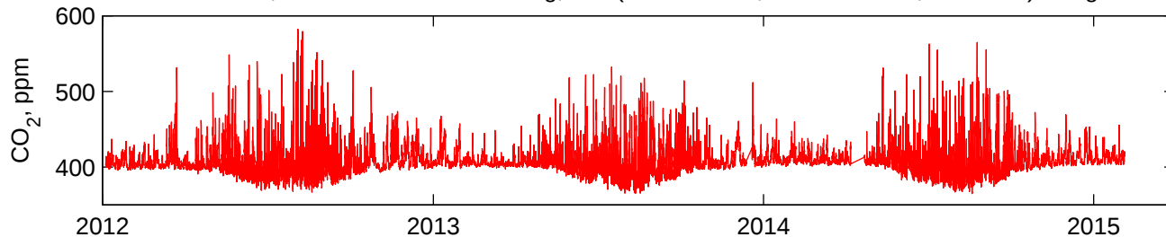
CARBON DIOXIDE, 20 min means. Lewisburg, PA. ( 40.944646^{\circ}\text{N} , 76.878855^{\circ}\text{W} , 165m asl). Height 50m agl.
