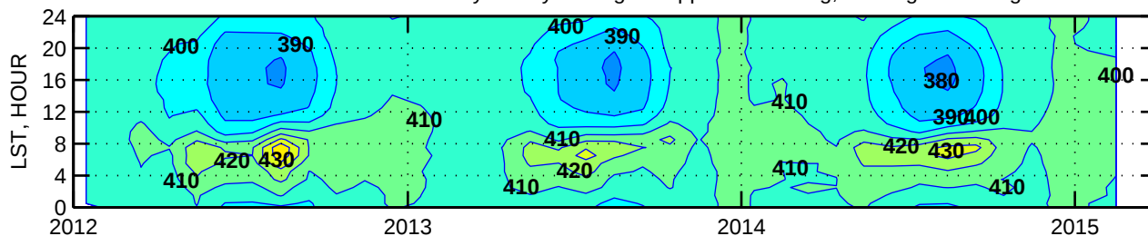
CARBON DIOXIDE Monthly/Hourly averages in ppm. Lewisburg, PA. Height=95m agl
