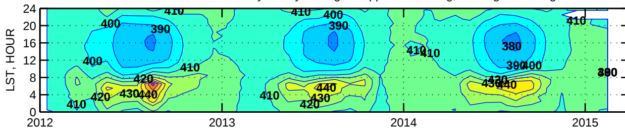
CARBON DIOXIDE Monthly/Hourly averages in ppm. Lewisburg, PA. Height=50m agl
