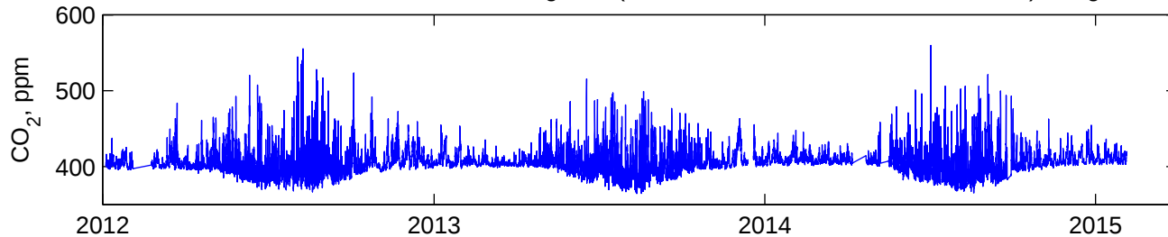
CARBON DIOXIDE, 20 min means. Lewisburg, PA. ( 40.944646^{\circ}\text{N} , 76.878855^{\circ}\text{W} , 165m asl). Height 95m agl.
