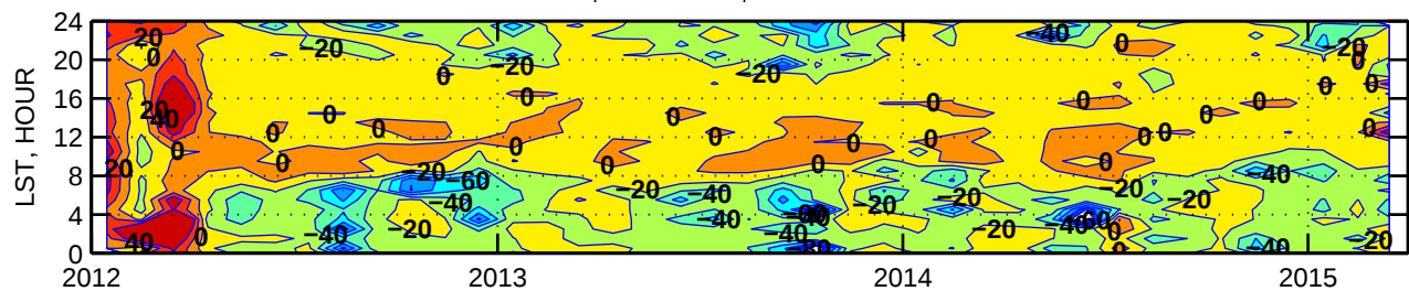
Difference \text{CH}_4(100\text{m}) - \text{CH}_4(50\text{m}) in ppb. Richmond, VA
