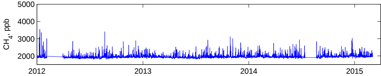
METHANE, 20 min means. Richmond, VA. (40.944646°N, 76.878855°W, 165m asl)). Height 100m agl.
