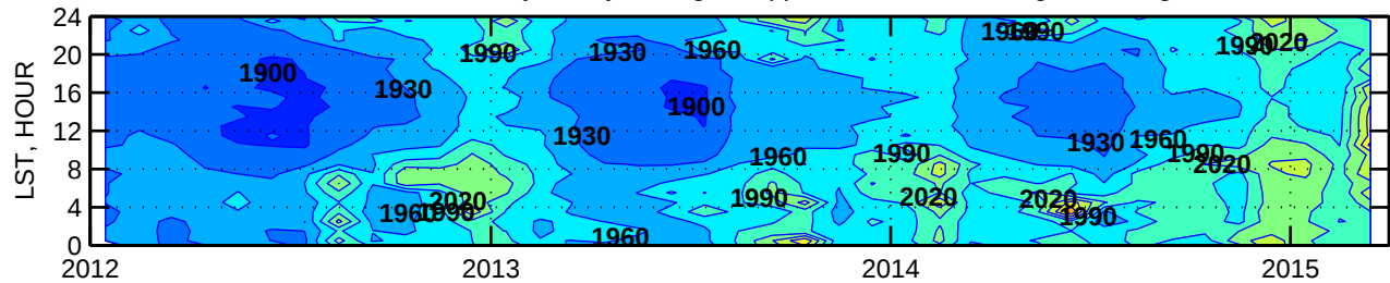
METHANE Monthly/Hourly averages in ppb. Richmond, VA. Height=50m agl
