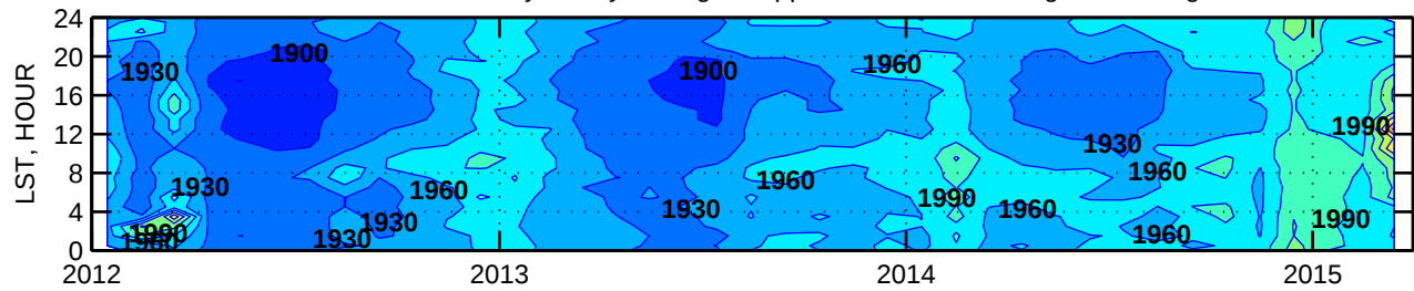
METHANE Monthly/Hourly averages in ppb. Richmond, VA. Height=100m agl
