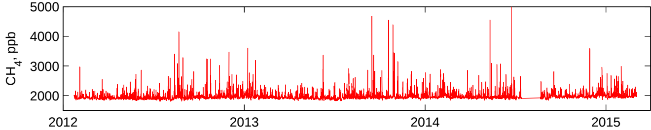
METHANE, 20 min means. Richmond, VA. (40.944646°N, 76.878855°W, 165m asl)). Height 50m agl.
