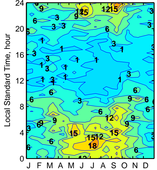
Beltsville, MD. LLJ Occurrence (%)
