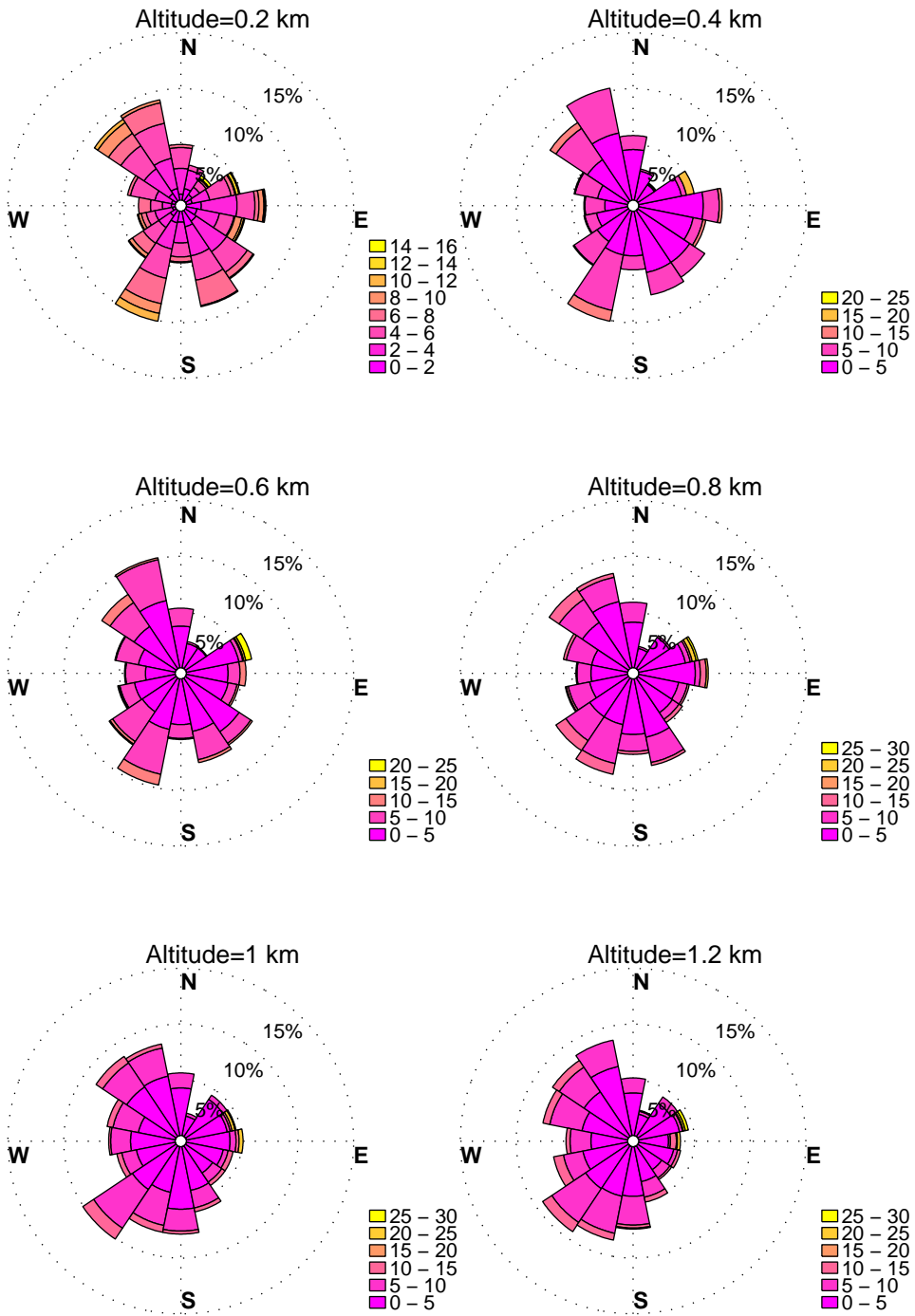
WINDROSES. BELTSVILLE, MD WIND PROFILER. AUGUST, HOURS: 12 pm to 15 pm DATA: FROM 1/2010 to 9/2014
