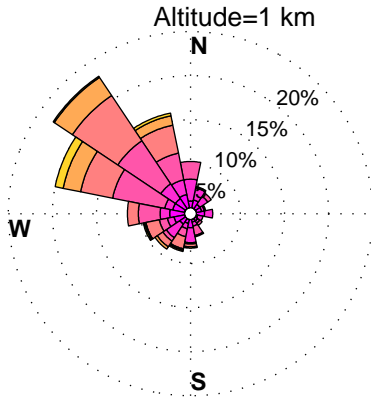
WINDROSES. BELTSVILLE, MD WIND PROFILER. FEBRUARY, HOURS: 12 am to 3 am DATA: FROM 1/2010 to 9/2014
