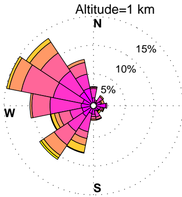
WINDROSES. BELTSVILLE, MD WIND PROFILER. JANUARY, HOURS: 12 pm to 15 pm DATA: FROM 1/2010 to 9/2014
