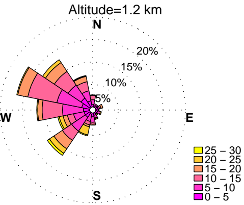
WINDROSES. BELTSVILLE, MD WIND PROFILER. JANUARY, HOURS: 12 pm to 15 pm DATA: FROM 1/2010 to 9/2014
