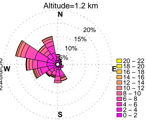
WINDROSES. BELTSVILLE, MD WIND PROFILER. JUNE, HOURS: 12 pm to 15 pm DATA: FROM 1/2010 to 9/2014
