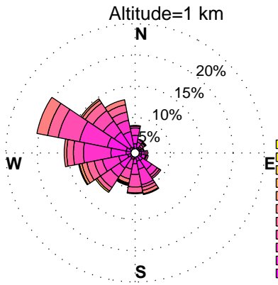
WINDROSES. BELTSVILLE, MD WIND PROFILER. JUNE, HOURS: 12 pm to 15 pm DATA: FROM 1/2010 to 9/2014
