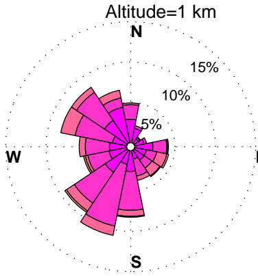
WINDROSES. BELTSVILLE, MD WIND PROFILER. MAY, HOURS: 12 pm to 15 pm DATA: FROM 1/2010 to 9/2014
