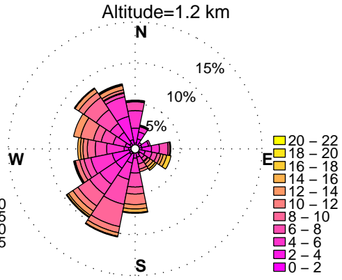
WINDROSES. BELTSVILLE, MD WIND PROFILER. MAY, HOURS: 12 pm to 15 pm DATA: FROM 1/2010 to 9/2014
