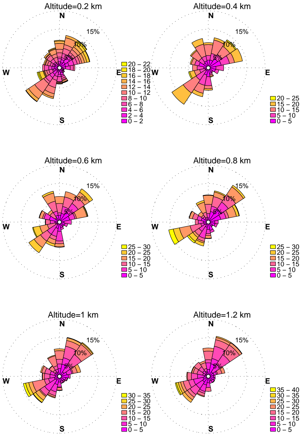
WINDROSES. BELTSVILLE, MD WIND PROFILER. NOVEMBER, HOURS: 12 am to 3 am DATA: FROM 1/2010 to 9/2014
