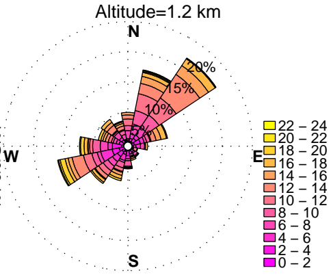
WINDROSES. BELTSVILLE, MD WIND PROFILER. SEPTEMBER, HOURS: 12 am to 3 am DATA: FROM 1/2010 to 9/2014
