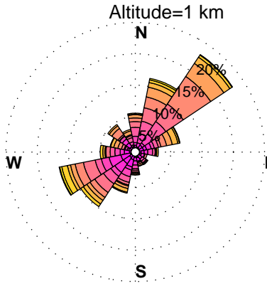
WINDROSES. BELTSVILLE, MD WIND PROFILER. SEPTEMBER, HOURS: 12 am to 3 am DATA: FROM 1/2010 to 9/2014
