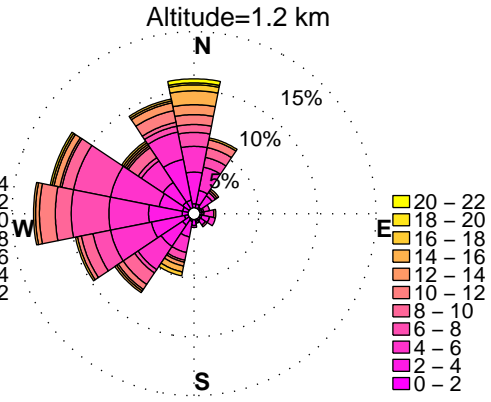
WINDROSES. BELTSVILLE, MD WIND PROFILER. JULY, HOURS: 10 am to 7 pm YEAR: 2010
