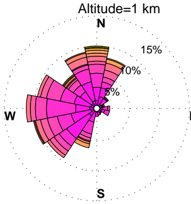
WINDROSES. BELTSVILLE, MD WIND PROFILER. JULY, HOURS: 10 am to 7 pm YEAR: 2010
