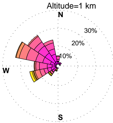
WINDROSES. BELTSVILLE, MD WIND PROFILER. JUNE, HOURS: 10 am to 7 pm YEAR: 2010
