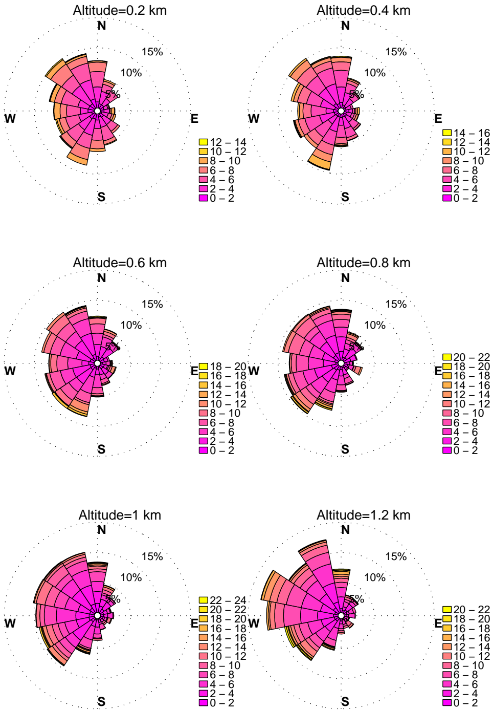
WINDROSES. BELTSVILLE, MD WIND PROFILER. MONTHS: JUNE to AUGUST, HOURS: 10 am to 7 pm YEAR: 2010
