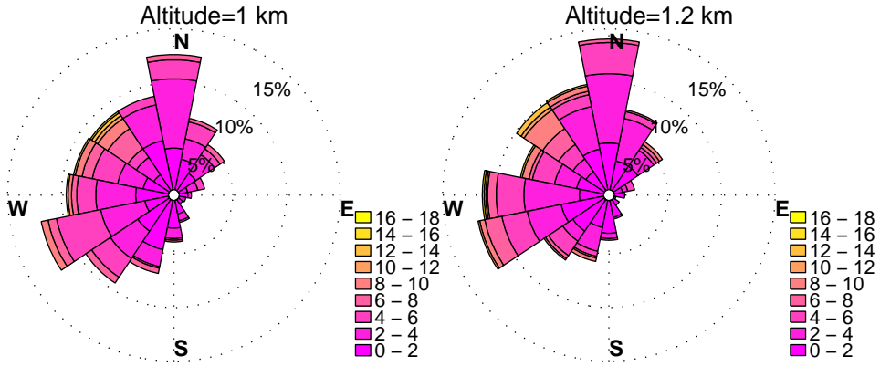
WINDROSES. BELTSVILLE, MD WIND PROFILER. JULY, HOURS: 10 am to 7 pm YEAR: 2011
