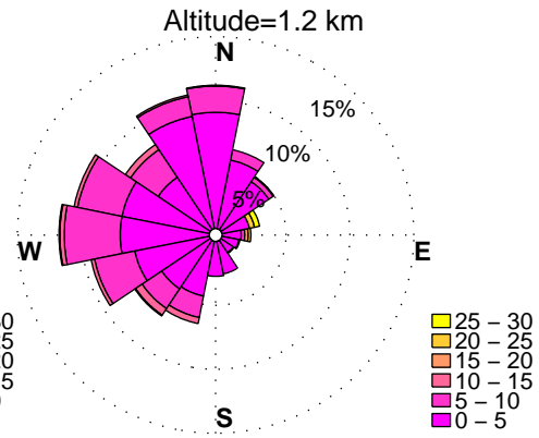
WINDROSES. BELTSVILLE, MD WIND PROFILER. MONTHS: JUNE to AUGUST, HOURS: 10 am to 7 pm YEAR: 2011
