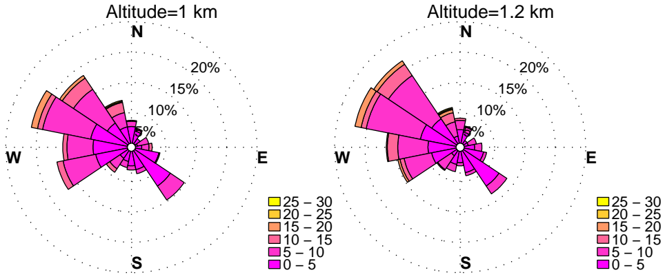
WINDROSES. BELTSVILLE, MD WIND PROFILER. JULY, HOURS: 10 am to 7 pm YEAR: 2012
