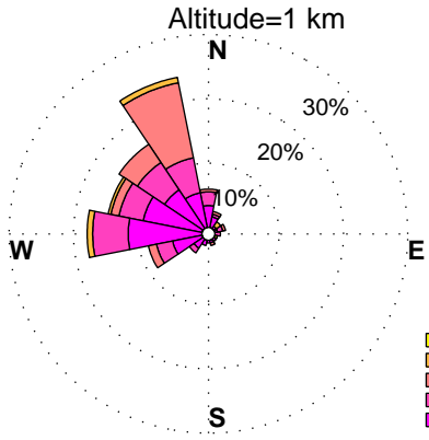
WINDROSES. BELTSVILLE, MD WIND PROFILER. JUNE, HOURS: 10 am to 7 pm YEAR: 2012
