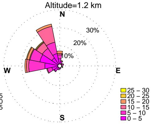
WINDROSES. BELTSVILLE, MD WIND PROFILER. JUNE, HOURS: 10 am to 7 pm YEAR: 2012
