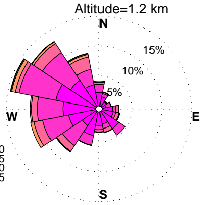
WINDROSES. BELTSVILLE, MD WIND PROFILER. MONTHS: JUNE to AUGUST, HOURS: 10 am to 7 pm YEAR: 2012
