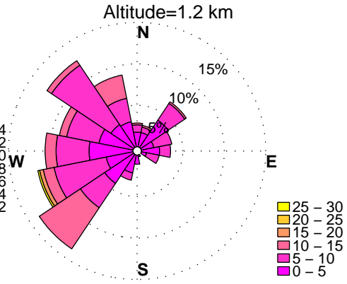
WINDROSES. BELTSVILLE, MD WIND PROFILER. AUGUST, HOURS: 10 am to 7 pm YEAR: 2013
