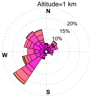
WINDROSES. BELTSVILLE, MD WIND PROFILER. AUGUST, HOURS: 10 am to 7 pm YEAR: 2013
