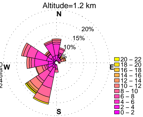
WINDROSES. BELTSVILLE, MD WIND PROFILER. JULY, HOURS: 10 am to 7 pm YEAR: 2013
