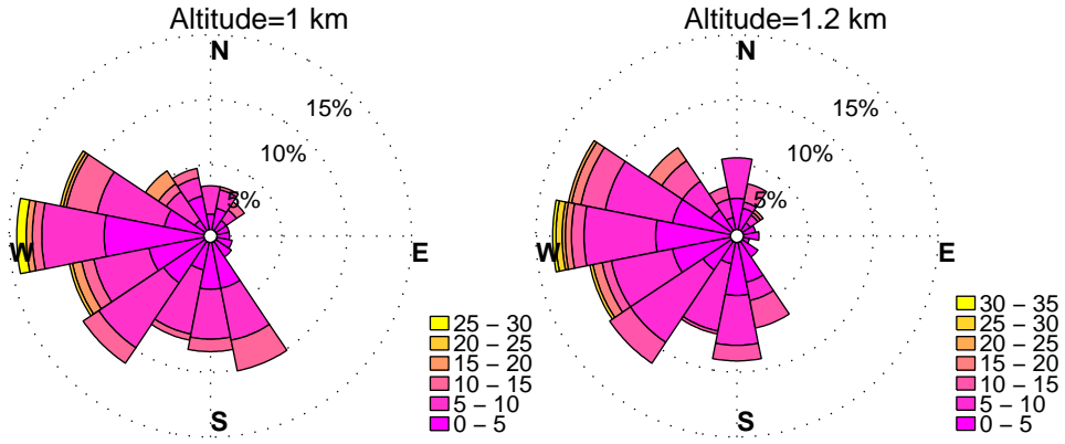
WINDROSES. BELTSVILLE, MD WIND PROFILER. JUNE, HOURS: 10 am to 7 pm YEAR: 2013
