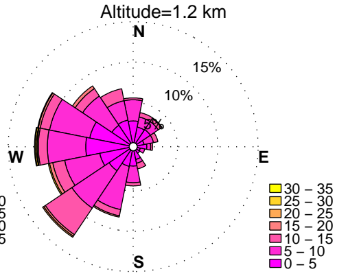
WINDROSES. BELTSVILLE, MD WIND PROFILER. MONTHS: JUNE to AUGUST, HOURS: 10 am to 7 pm YEAR: 2013
