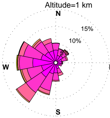
WINDROSES. BELTSVILLE, MD WIND PROFILER. MONTHS: JUNE to AUGUST, HOURS: 10 am to 7 pm YEAR: 2013
